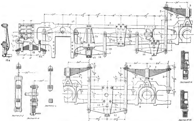
Figs. 1615-1621. Spring Rigging for Atlantic (1-4-2) Locomotive. P. R. R.
